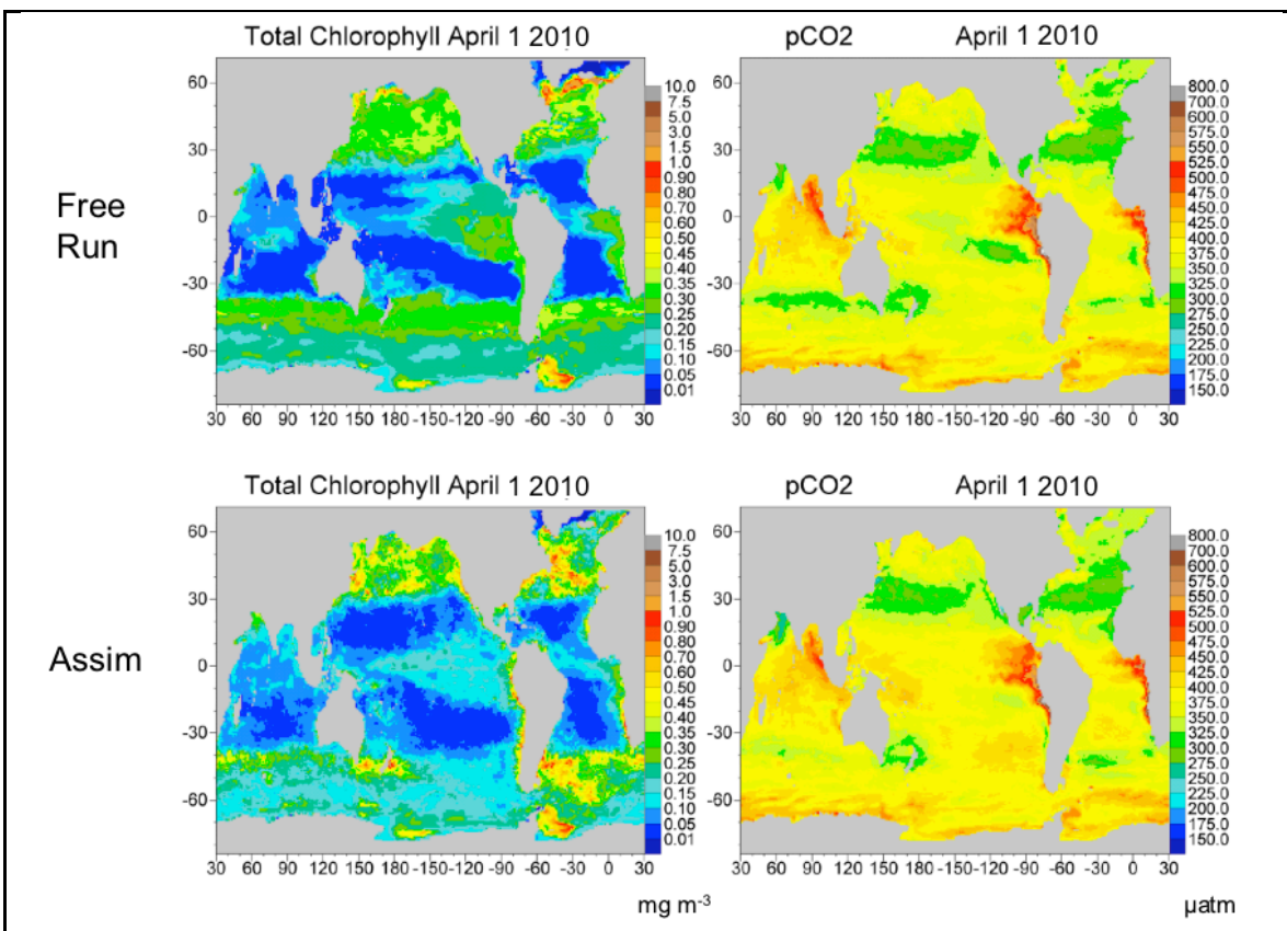
Fig. 4.4.d. Free run and assimilated chlorophyll, with resulting pCO 2 distributions.
